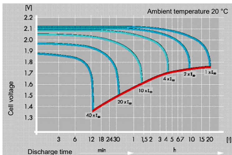
Fig. 1: Discharge characteristics 5 NSV
